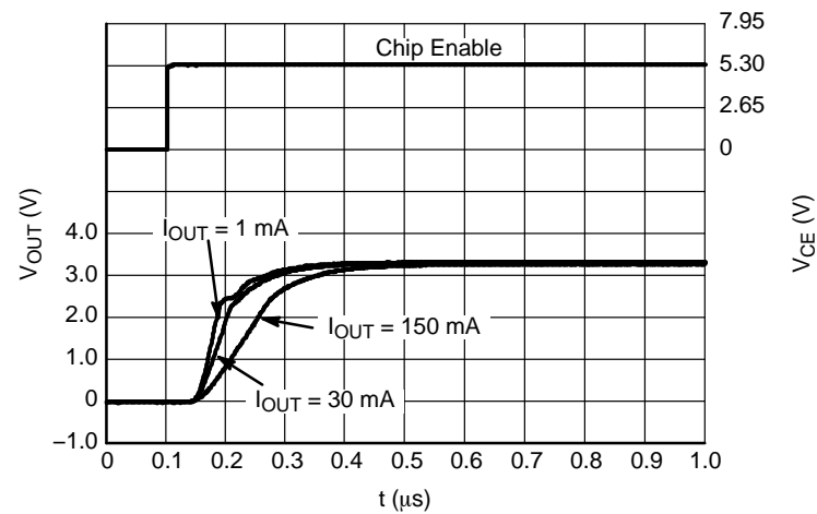
Figure 42. Start-up, 3.3 V Version, V_{IN} = 5.3 V
